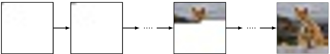
Figure 12.24 An illustration of how an image can be sampled from an autoregressive model. The first pixel is sampled from the marginal distribution p(x_{11}) , the second pixel from the conditional distribution p(x_{12} | x_{11}) , and so on in raster scan order until we have a complete image.
